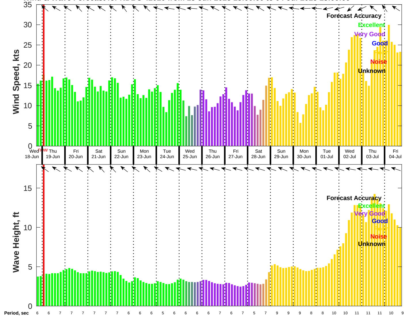
Wind & Wave Forecast for NDBC 42020 from 18-Jun-2025 18:00:00 to 04-Jul-2025 18:00:00
