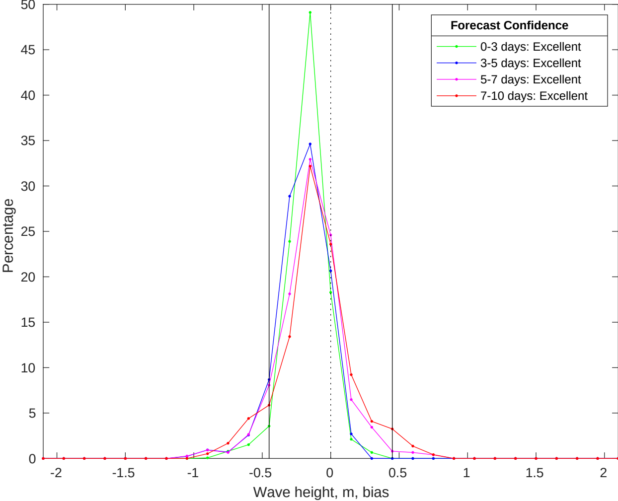
NDBC 42035 vs CMEMS Waves Bias Histogram: 19-Jun-2025
