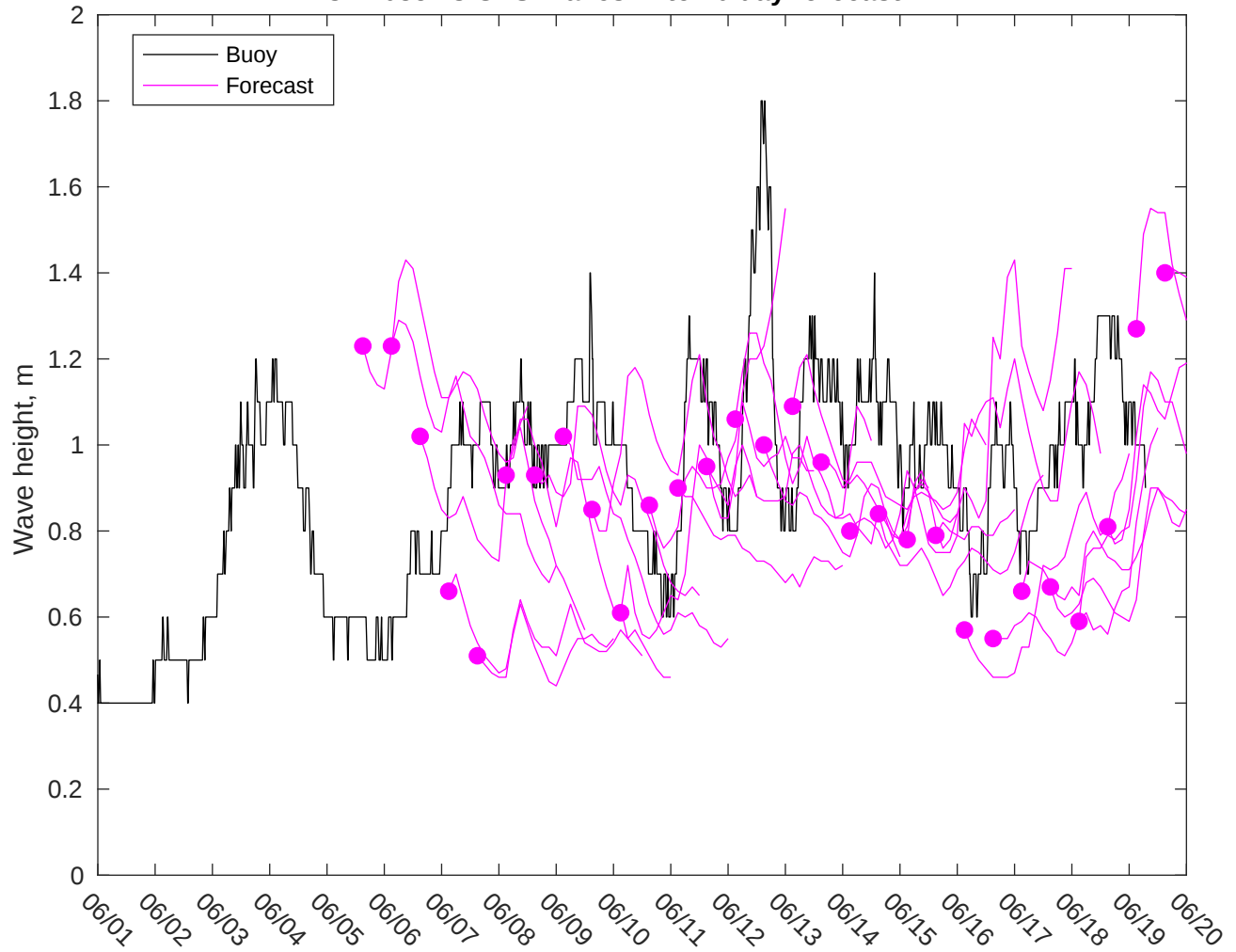
NDBC 42035 vs GFS Waves: 7 to 10 day forecast
