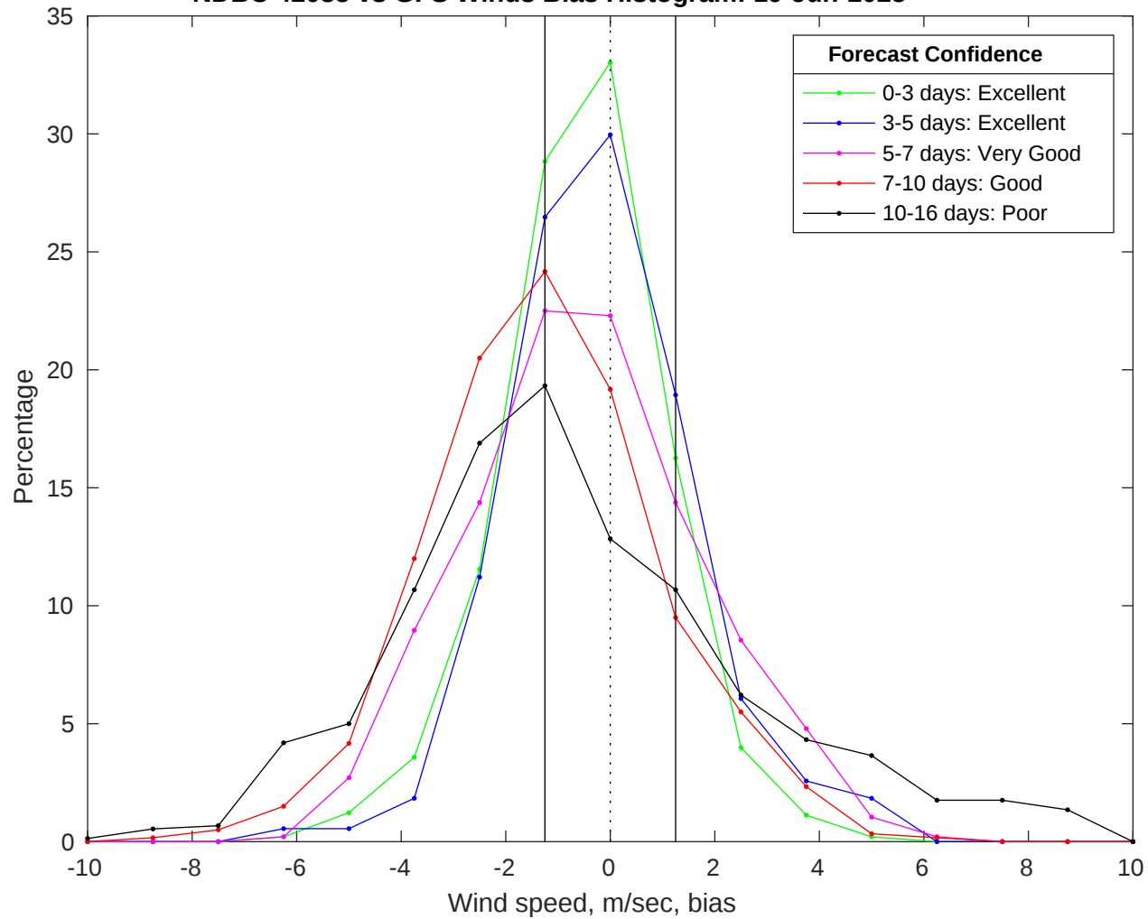
NDBC 42035 vs GFS Winds Bias Histogram: 19-Jun-2025
