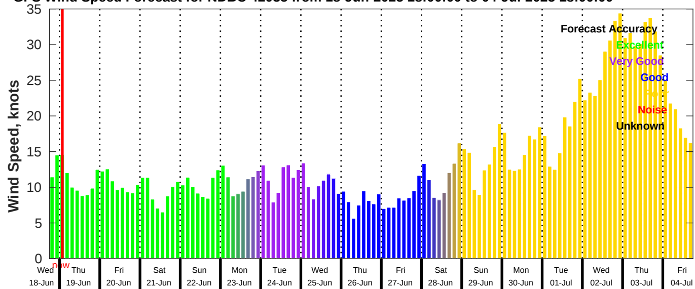
GFS Wind Speed Forecast for NDBC 42035 from 18-Jun-2025 18:00:00 to 04-Jul-2025 18:00:00
