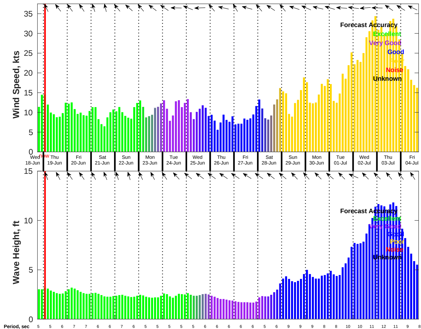
Wind & Wave Forecast for NDBC 42035 from 18-Jun-2025 18:00:00 to 04-Jul-2025 18:00:00
