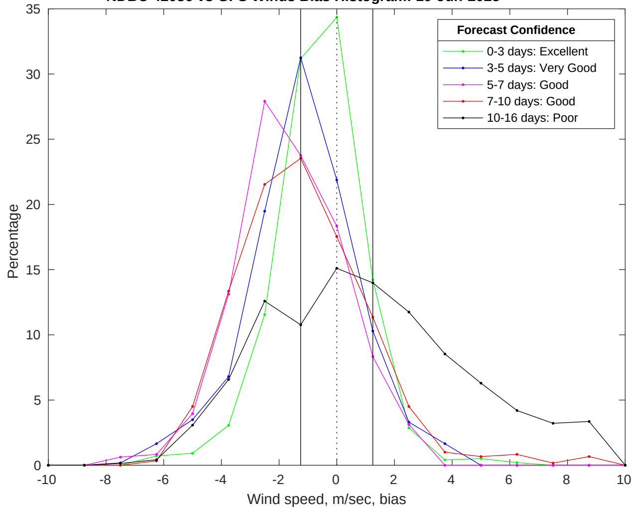
NDBC 42036 vs GFS Winds Bias Histogram: 19-Jun-2025
