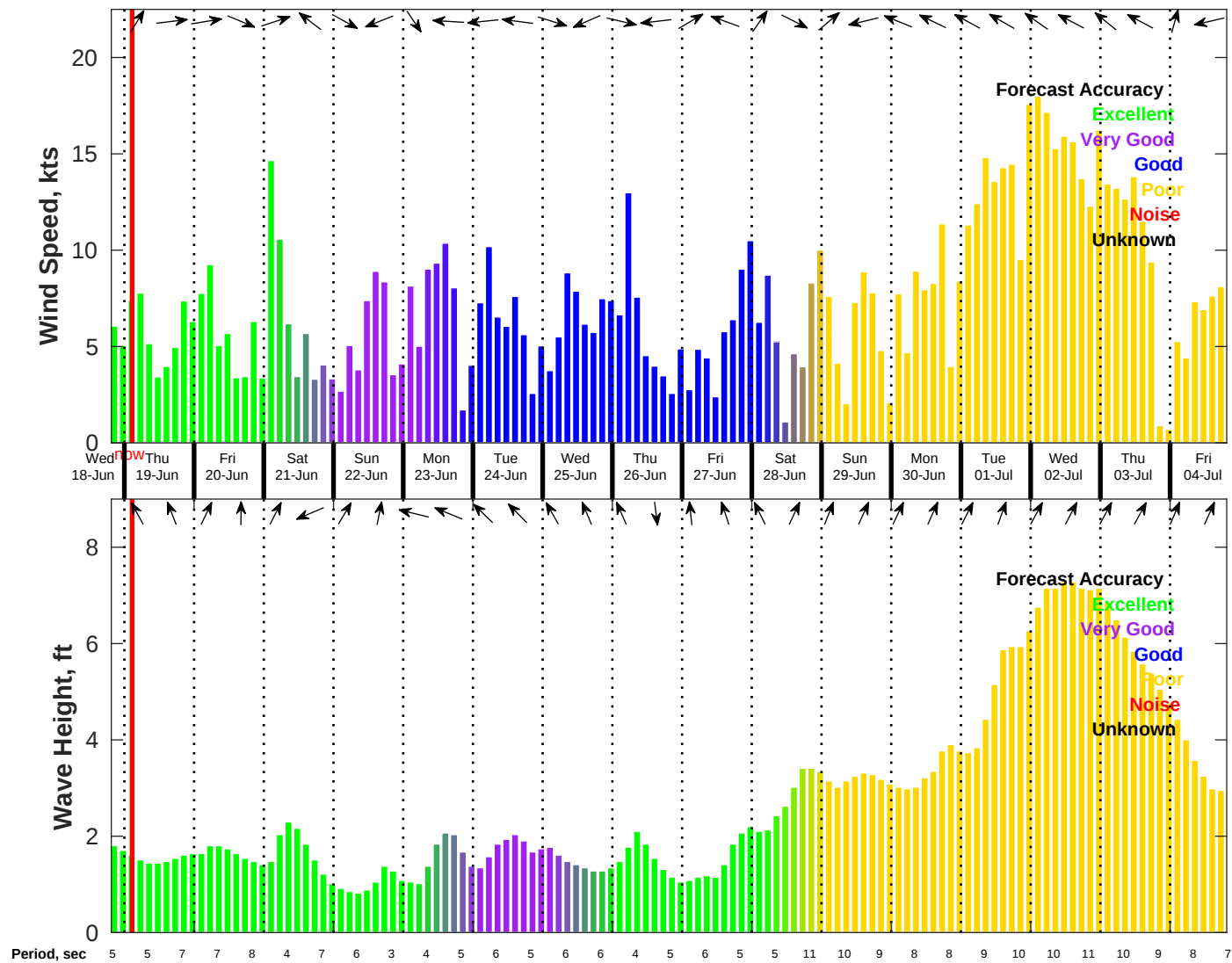
Wind & Wave Forecast for NDBC 42036 from 18-Jun-2025 19:00:00 to 04-Jul-2025 19:00:00
