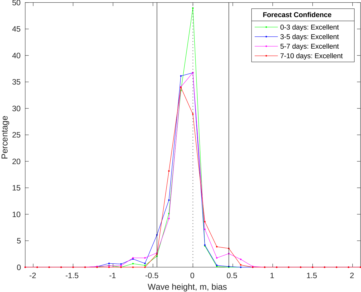
NDBC 42040 vs CMEMS Waves Bias Histogram: 19-Jun-2025
