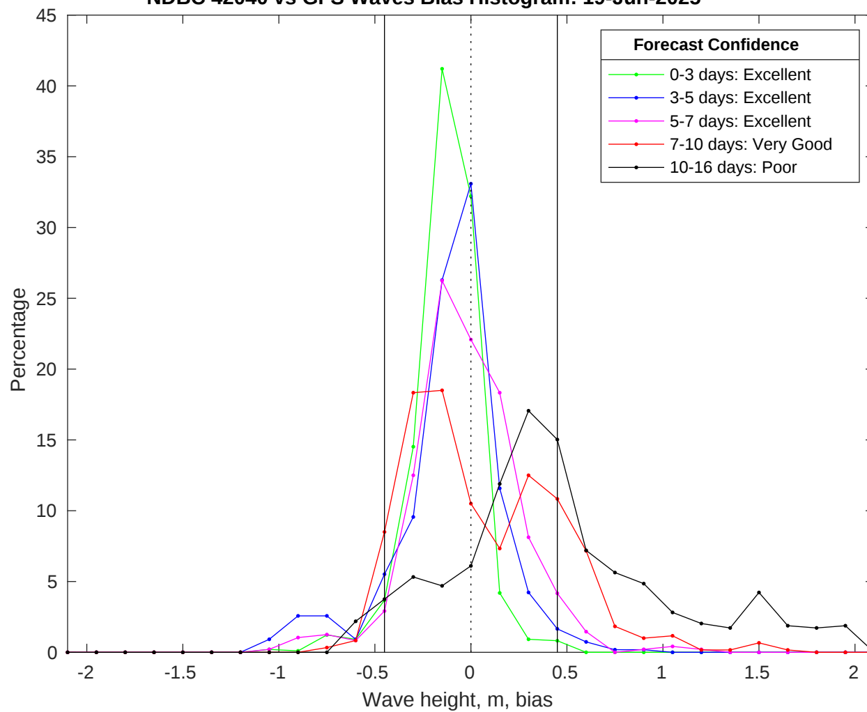
NDBC 42040 vs GFS Waves Bias Histogram: 19-Jun-2025
