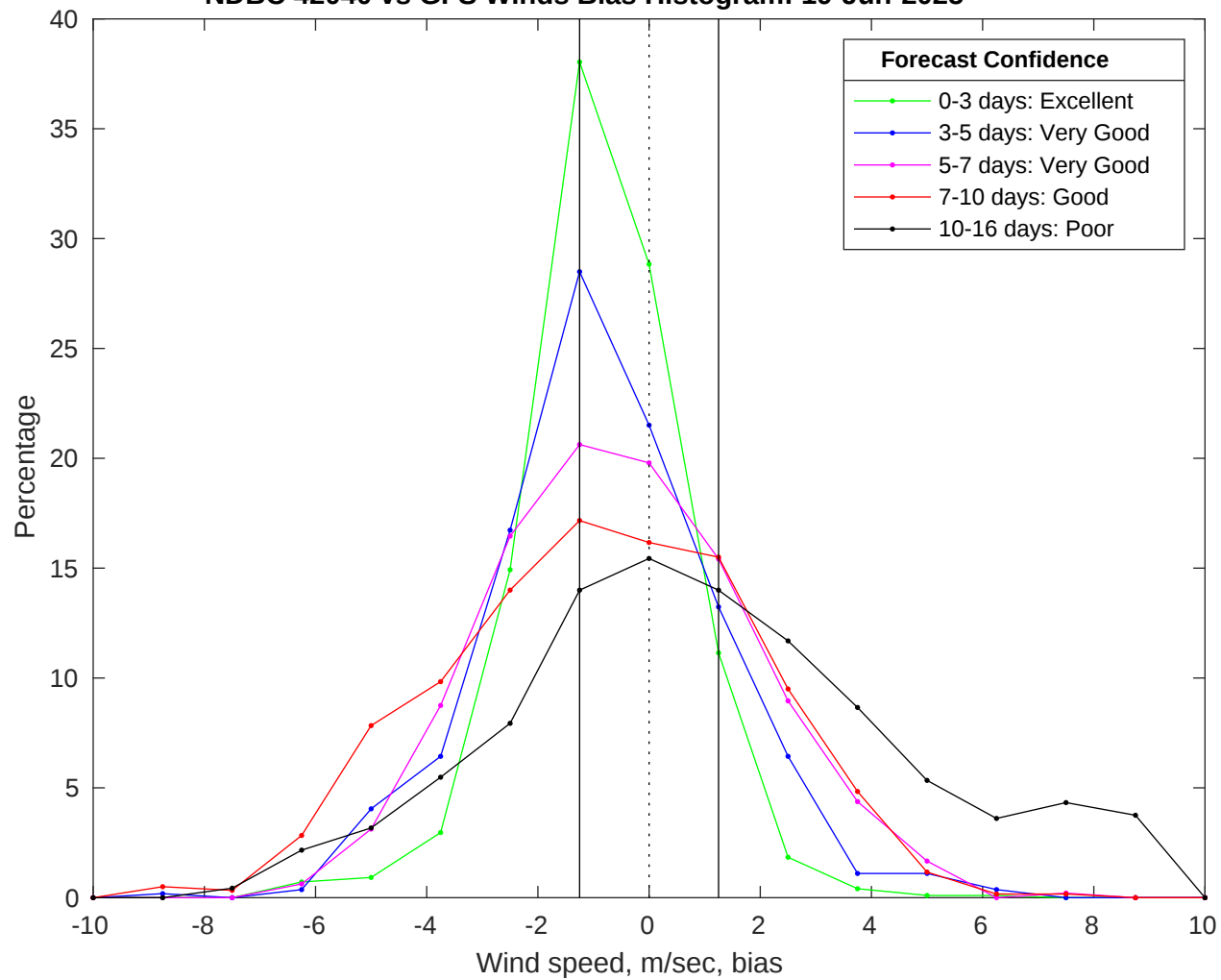
NDBC 42040 vs GFS Winds Bias Histogram: 19-Jun-2025
