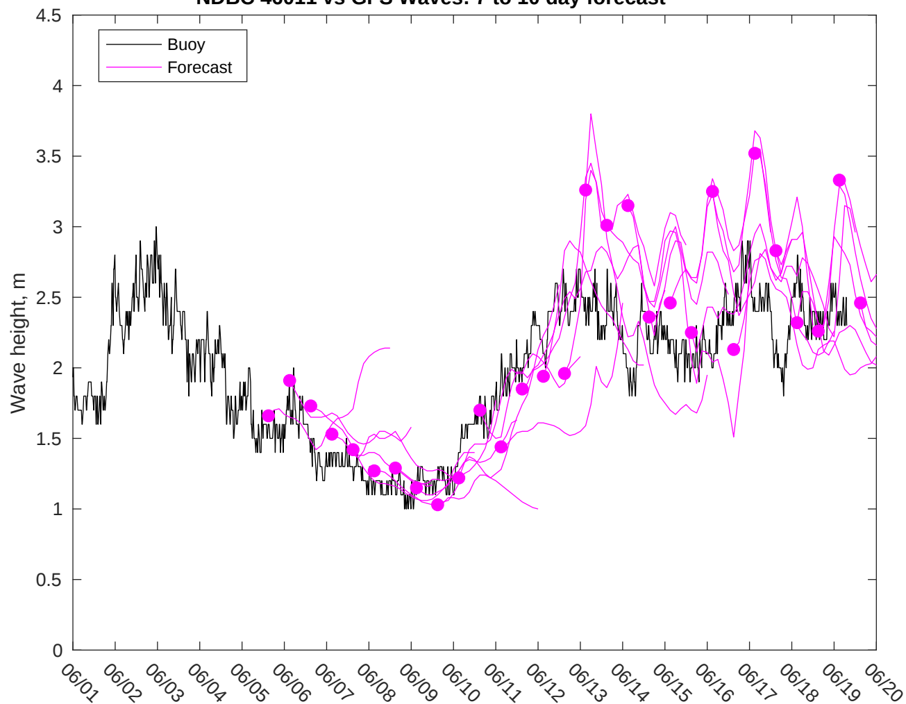
NDBC 46011 vs GFS Waves: 7 to 10 day forecast
