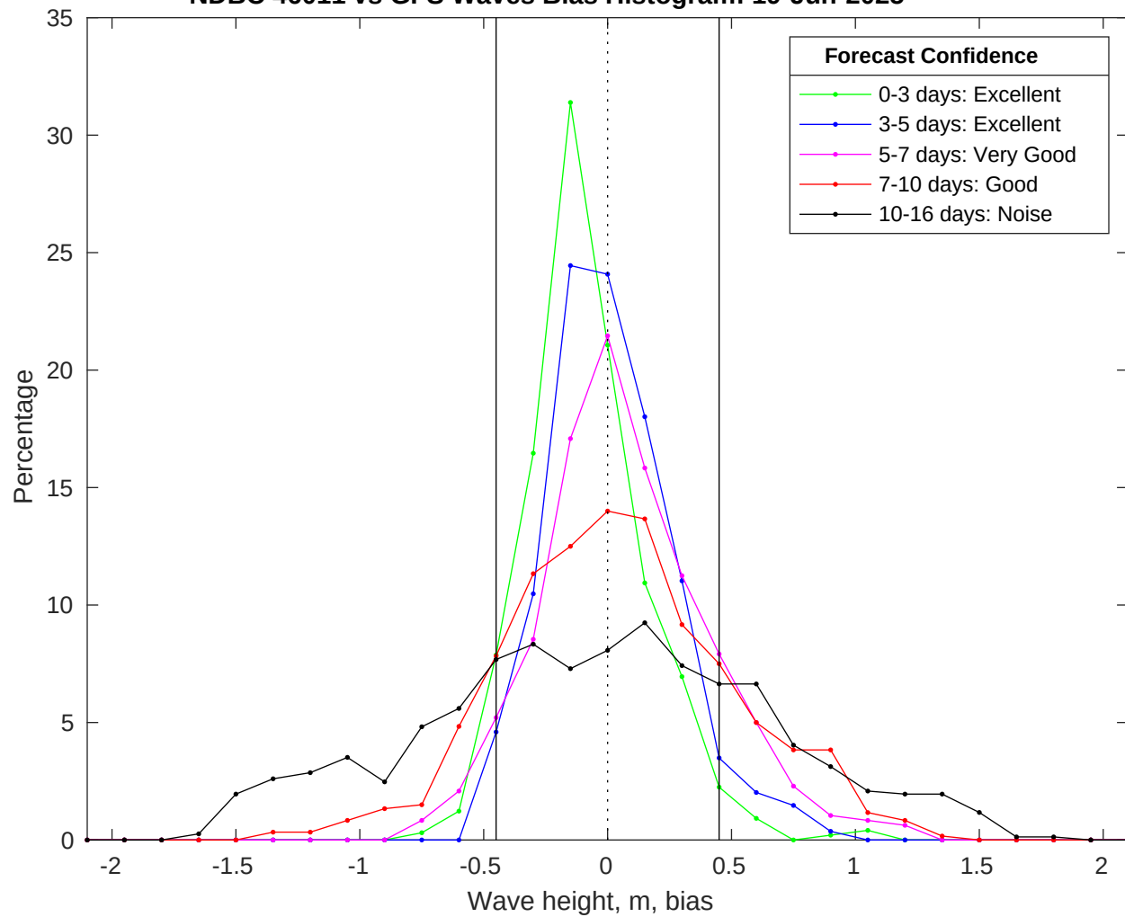
NDBC 46011 vs GFS Waves Bias Histogram: 19-Jun-2025
