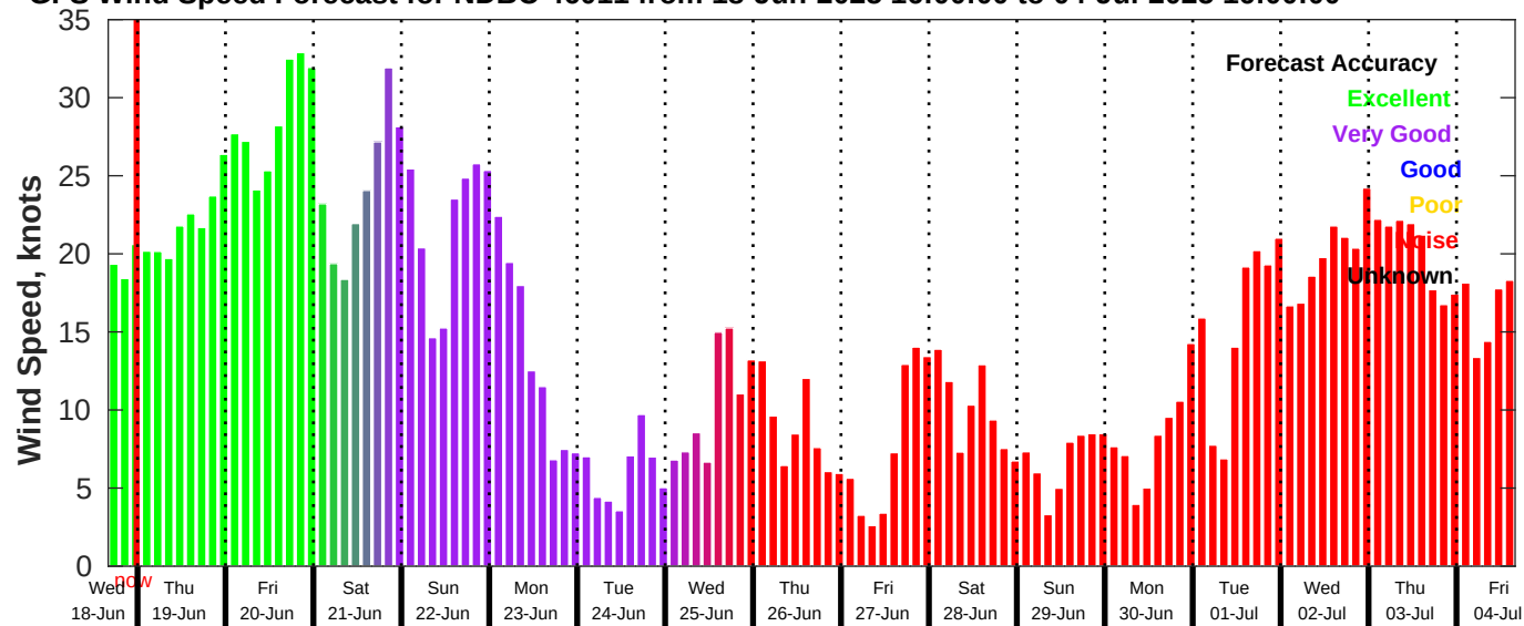
GFS Wind Speed Forecast for NDBC 46011 from 18-Jun-2025 16:00:00 to 04-Jul-2025 16:00:00
