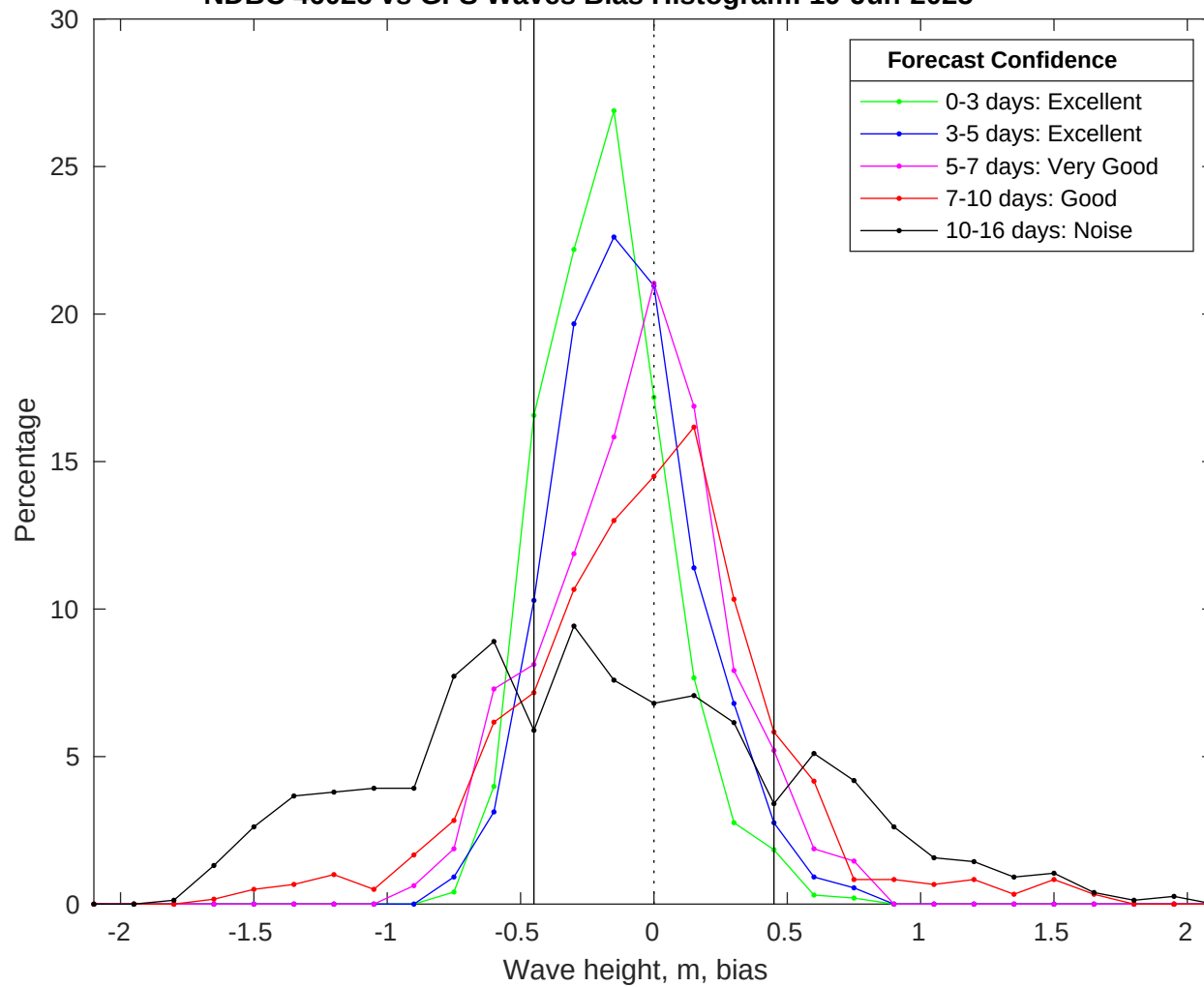
NDBC 46028 vs GFS Waves Bias Histogram: 19-Jun-2025
