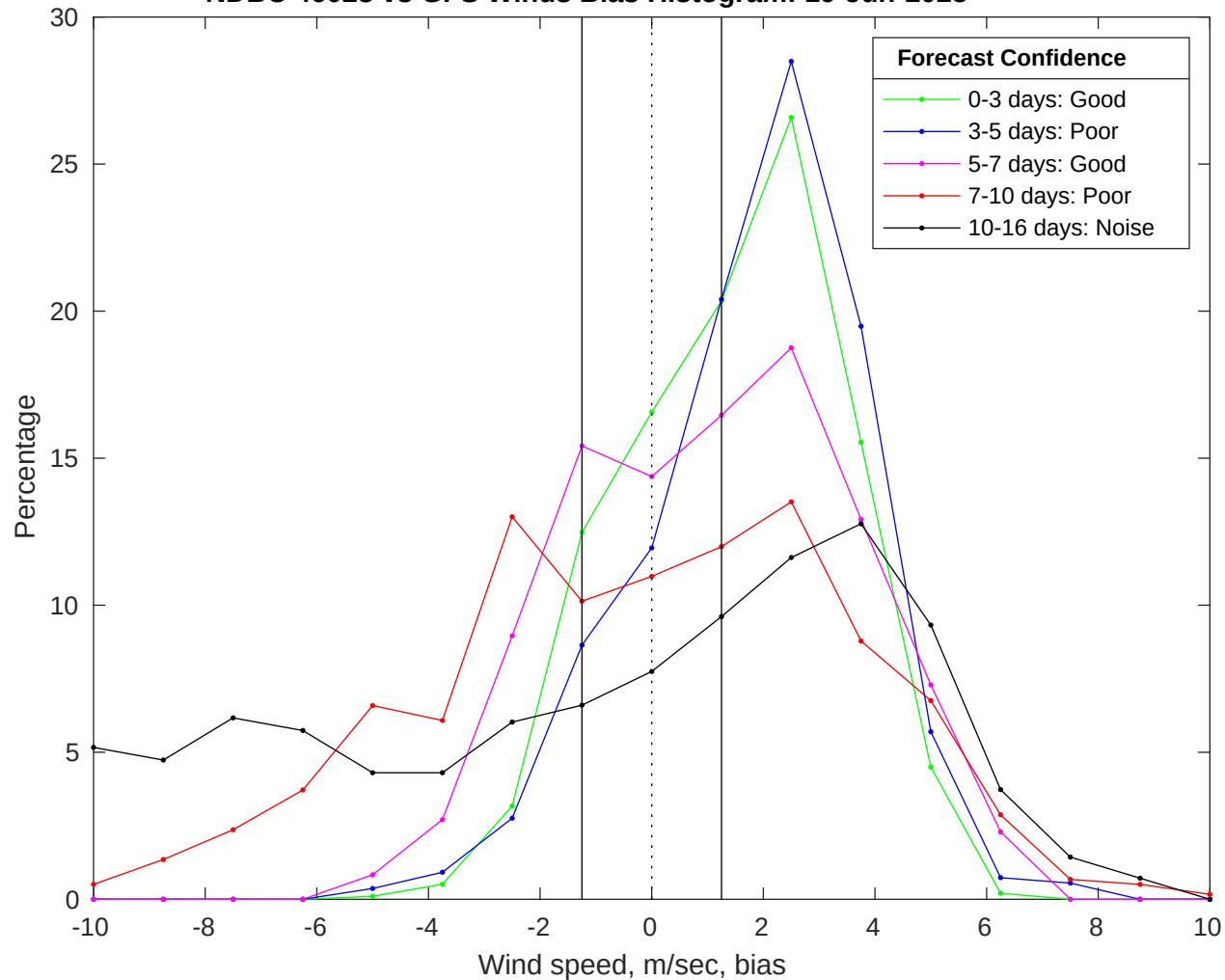
NDBC 46028 vs GFS Winds Bias Histogram: 19-Jun-2025
