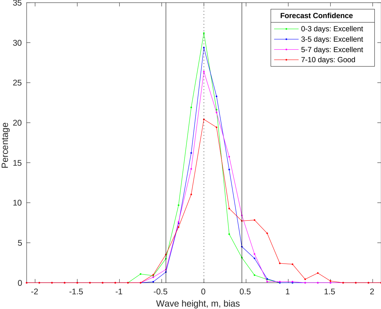
NDBC 46054 vs CMEMS Waves Bias Histogram: 19-Jun-2025
