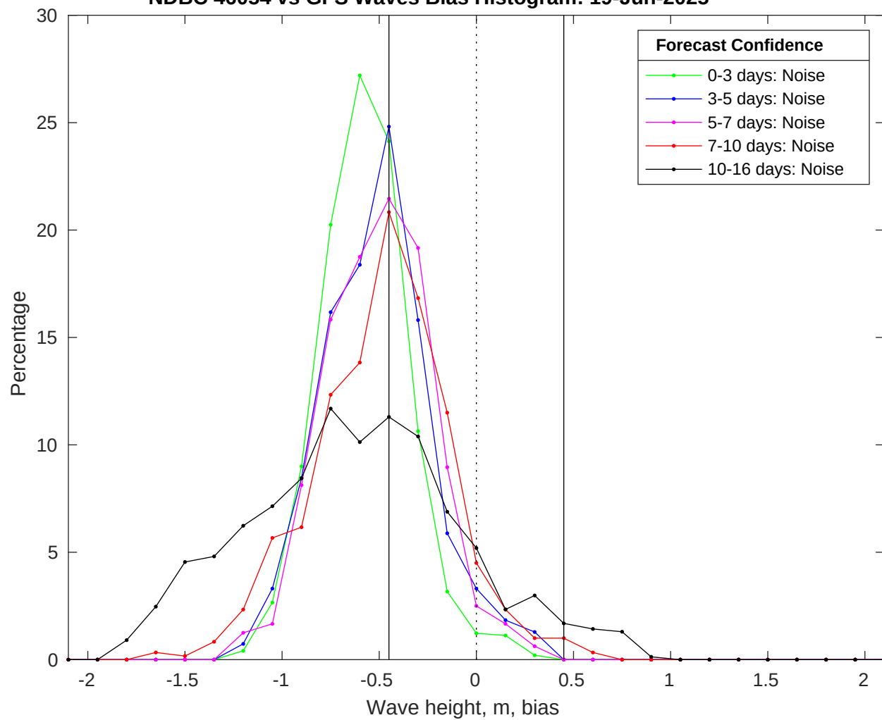
NDBC 46054 vs GFS Waves Bias Histogram: 19-Jun-2025
