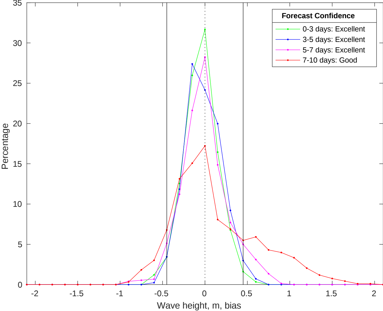
NDBC 46069 vs CMEMS Waves Bias Histogram: 19-Jun-2025
