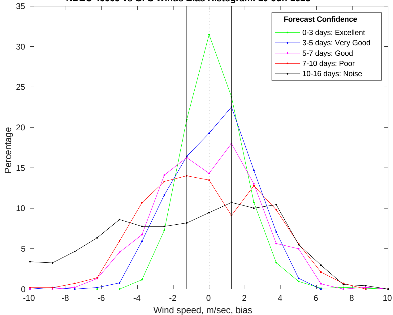
NDBC 46069 vs GFS Winds Bias Histogram: 19-Jun-2025
