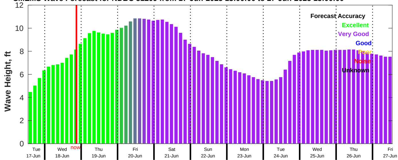
CMEMS Wave Forecast for NDBC 51209 from 17-Jun-2025 13:00:00 to 27-Jun-2025 13:00:00
