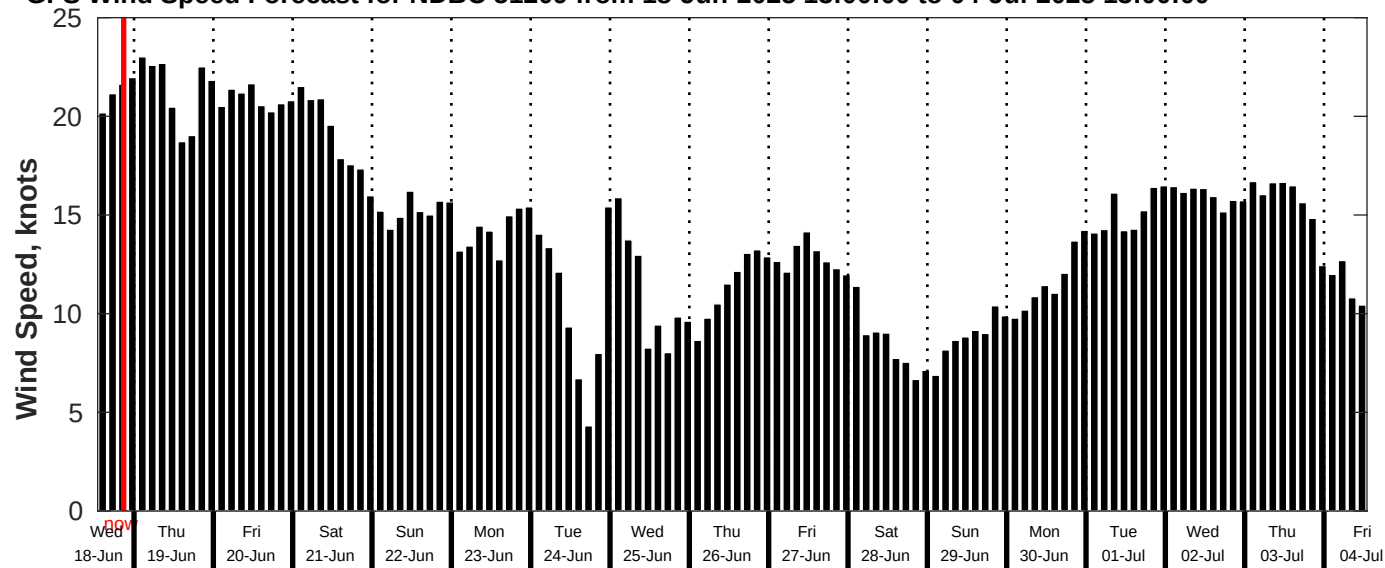
GFS Wind Speed Forecast for NDBC 51209 from 18-Jun-2025 13:00:00 to 04-Jul-2025 13:00:00
