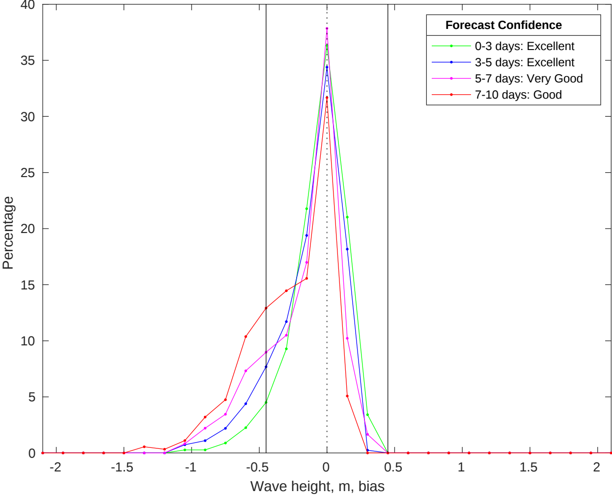
NDBC 52212 vs CMEMS Waves Bias Histogram: 19-Jun-2025
