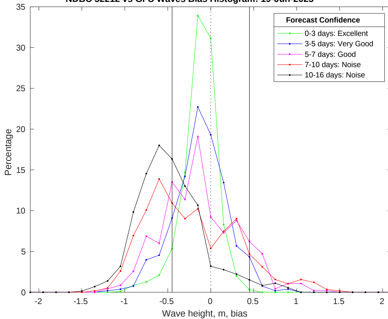
NDBC 52212 vs GFS Waves Bias Histogram: 19-Jun-2025
