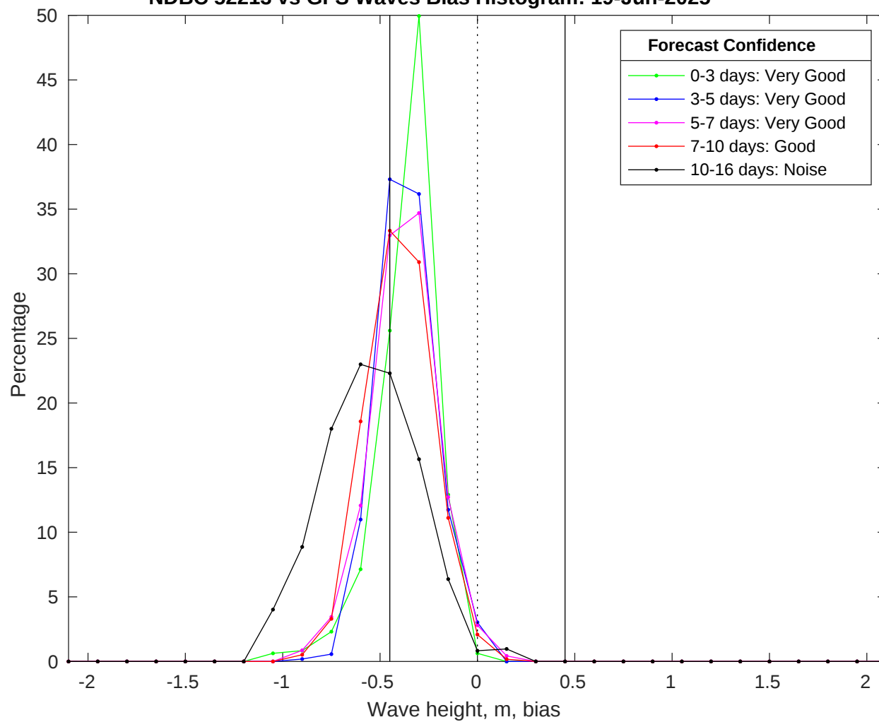
NDBC 52213 vs GFS Waves Bias Histogram: 19-Jun-2025
