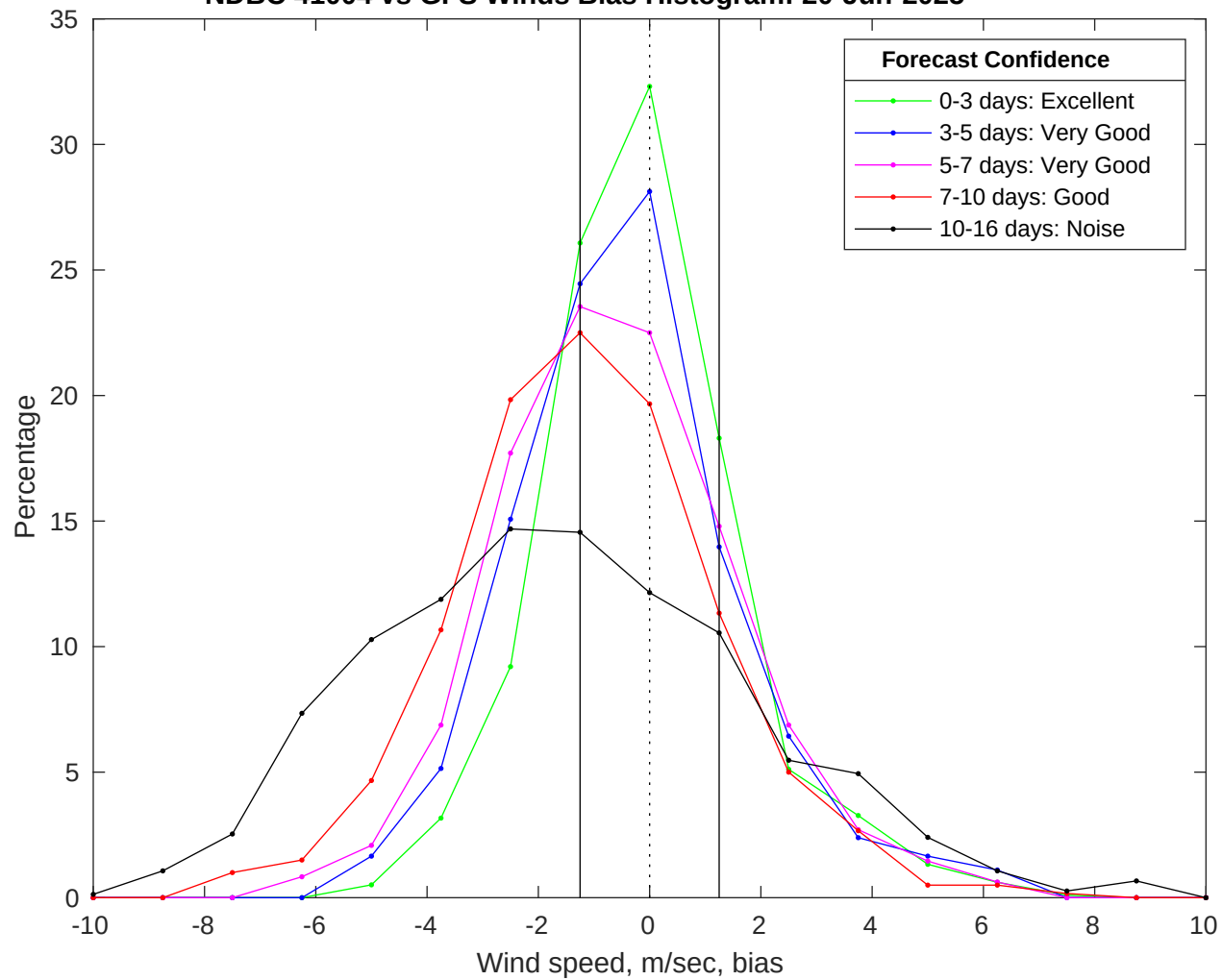
NDBC 41004 vs GFS Winds Bias Histogram: 20-Jun-2025
