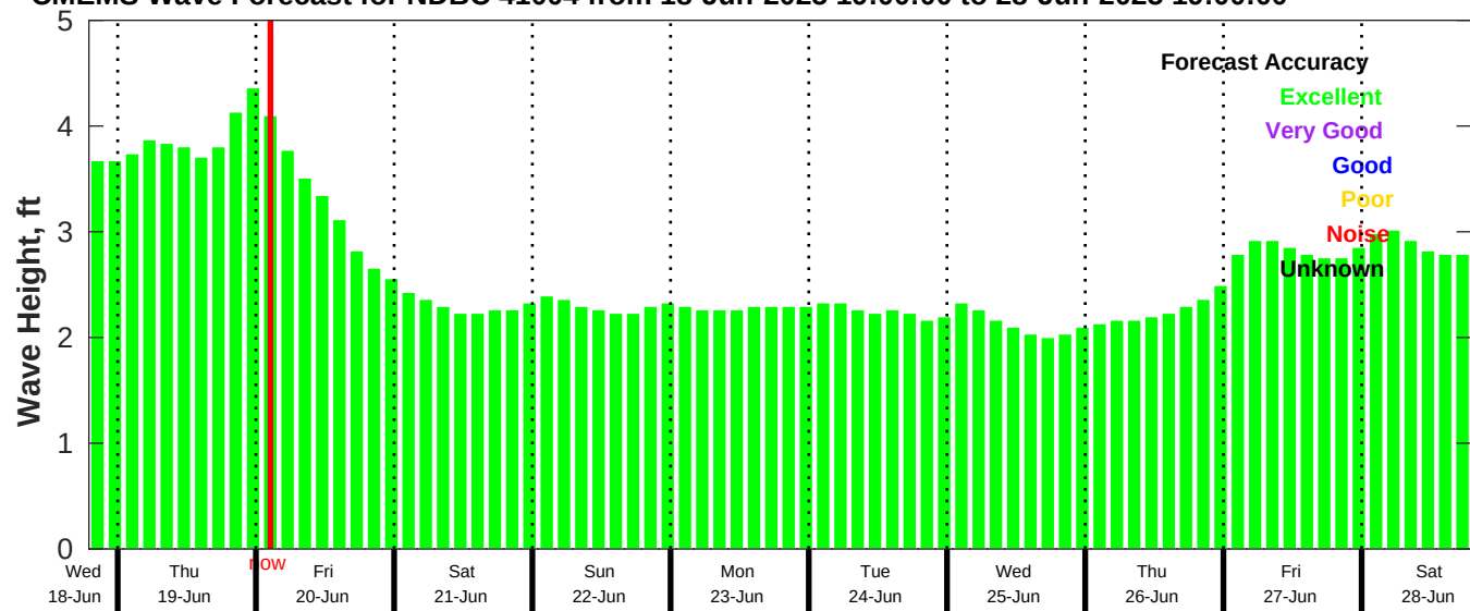
CMEMS Wave Forecast for NDBC 41004 from 18-Jun-2025 19:00:00 to 28-Jun-2025 19:00:00
