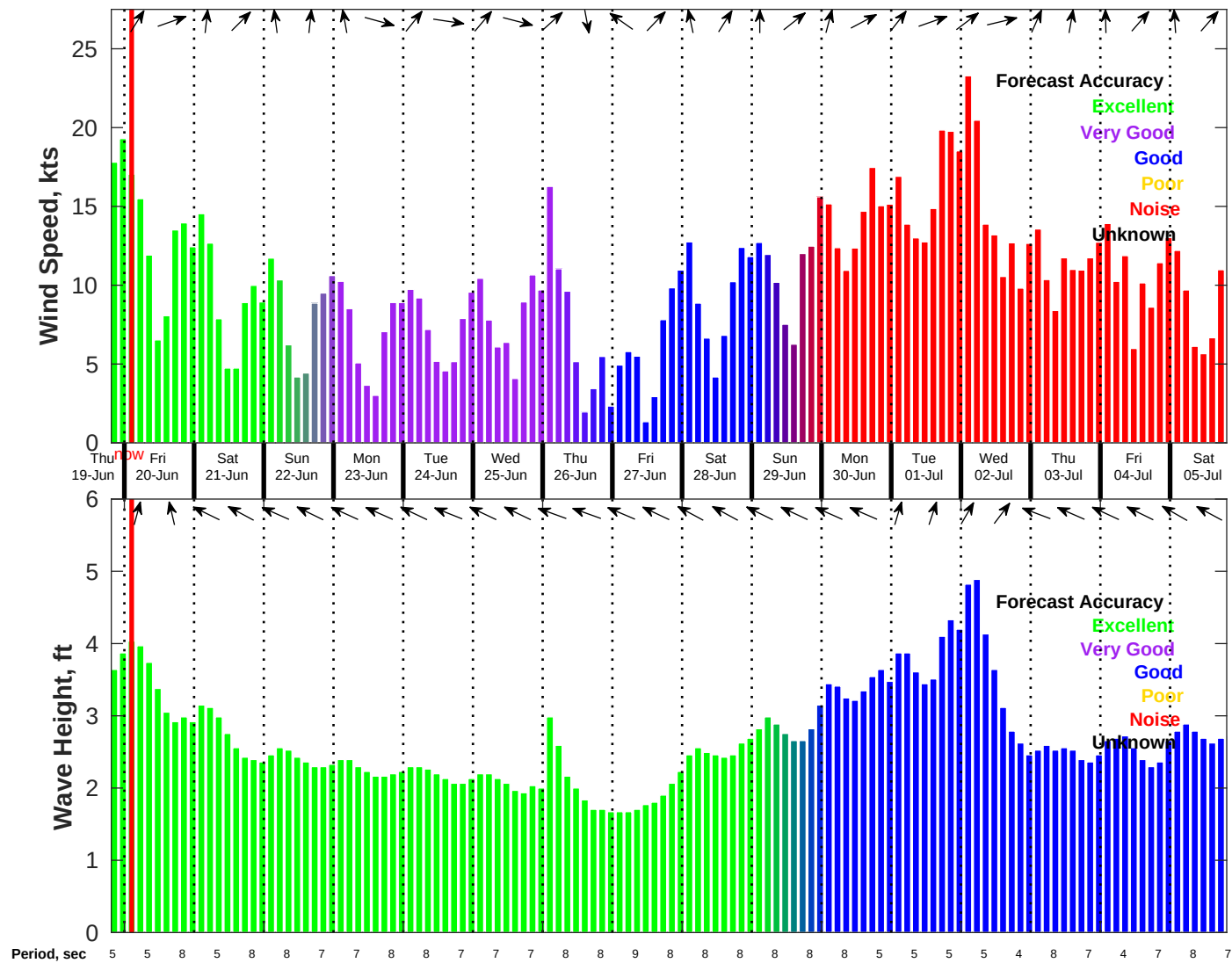
Wind & Wave Forecast for NDBC 41004 from 19-Jun-2025 19:00:00 to 05-Jul-2025 19:00:00
