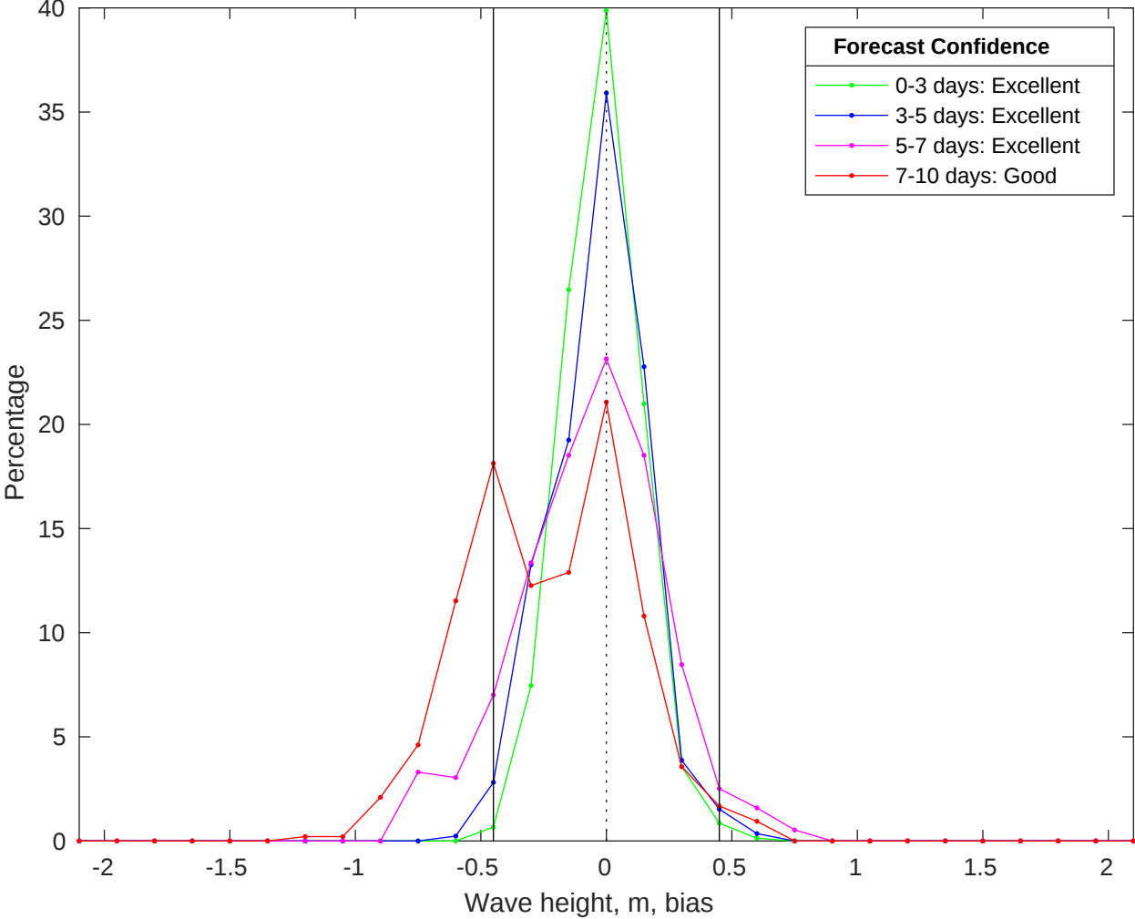
NDBC 41013 vs CMEMS Waves Bias Histogram: 20-Jun-2025
