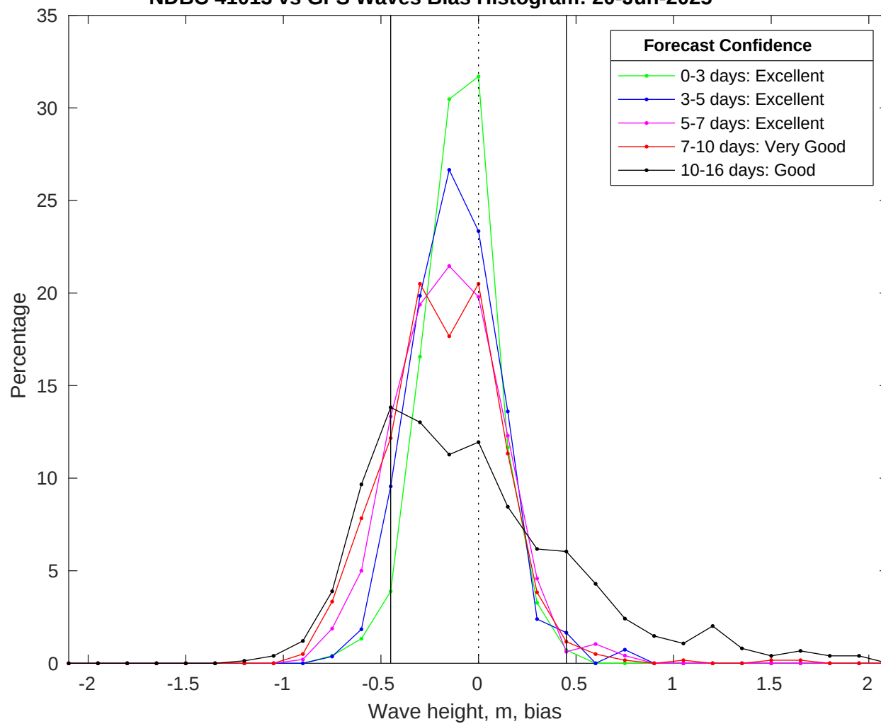
NDBC 41013 vs GFS Waves Bias Histogram: 20-Jun-2025
