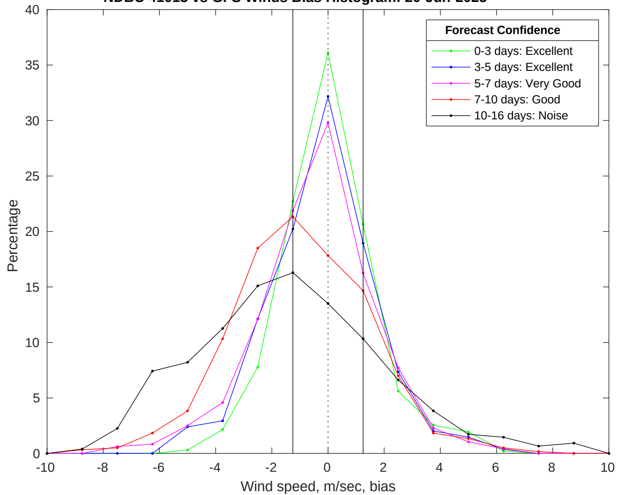
NDBC 41013 vs GFS Winds Bias Histogram: 20-Jun-2025
