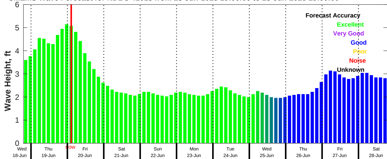
CMEMS Wave Forecast for NDBC 41013 from 18-Jun-2025 19:00:00 to 28-Jun-2025 19:00:00
