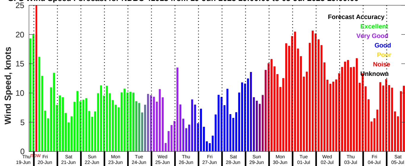
GFS Wind Speed Forecast for NDBC 41013 from 19-Jun-2025 19:00:00 to 05-Jul-2025 19:00:00
