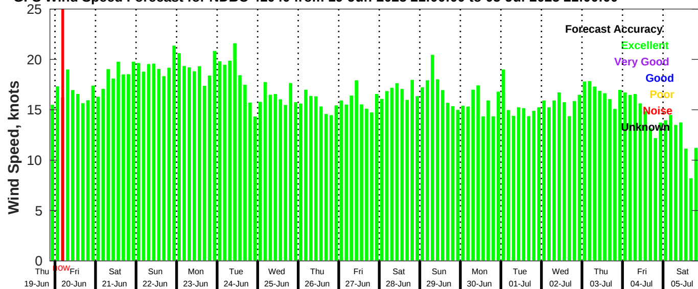
GFS Wind Speed Forecast for NDBC 41040 from 19-Jun-2025 21:00:00 to 05-Jul-2025 21:00:00
