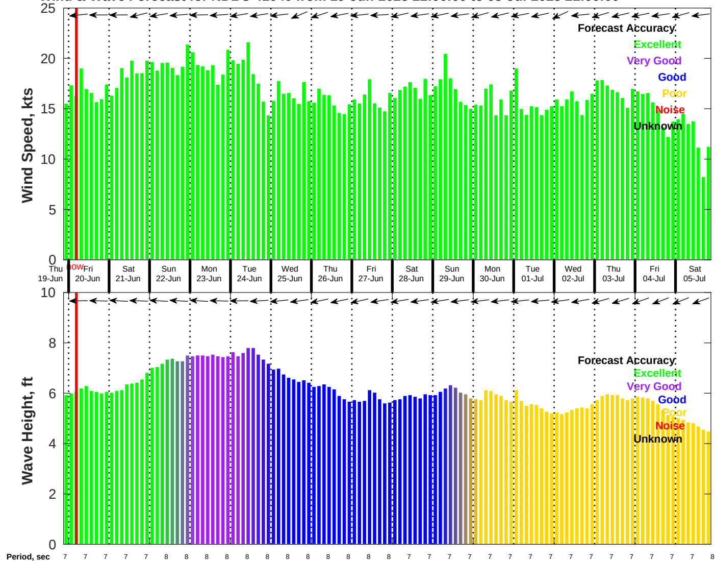
Wind & Wave Forecast for NDBC 41040 from 19-Jun-2025 21:00:00 to 05-Jul-2025 21:00:00
