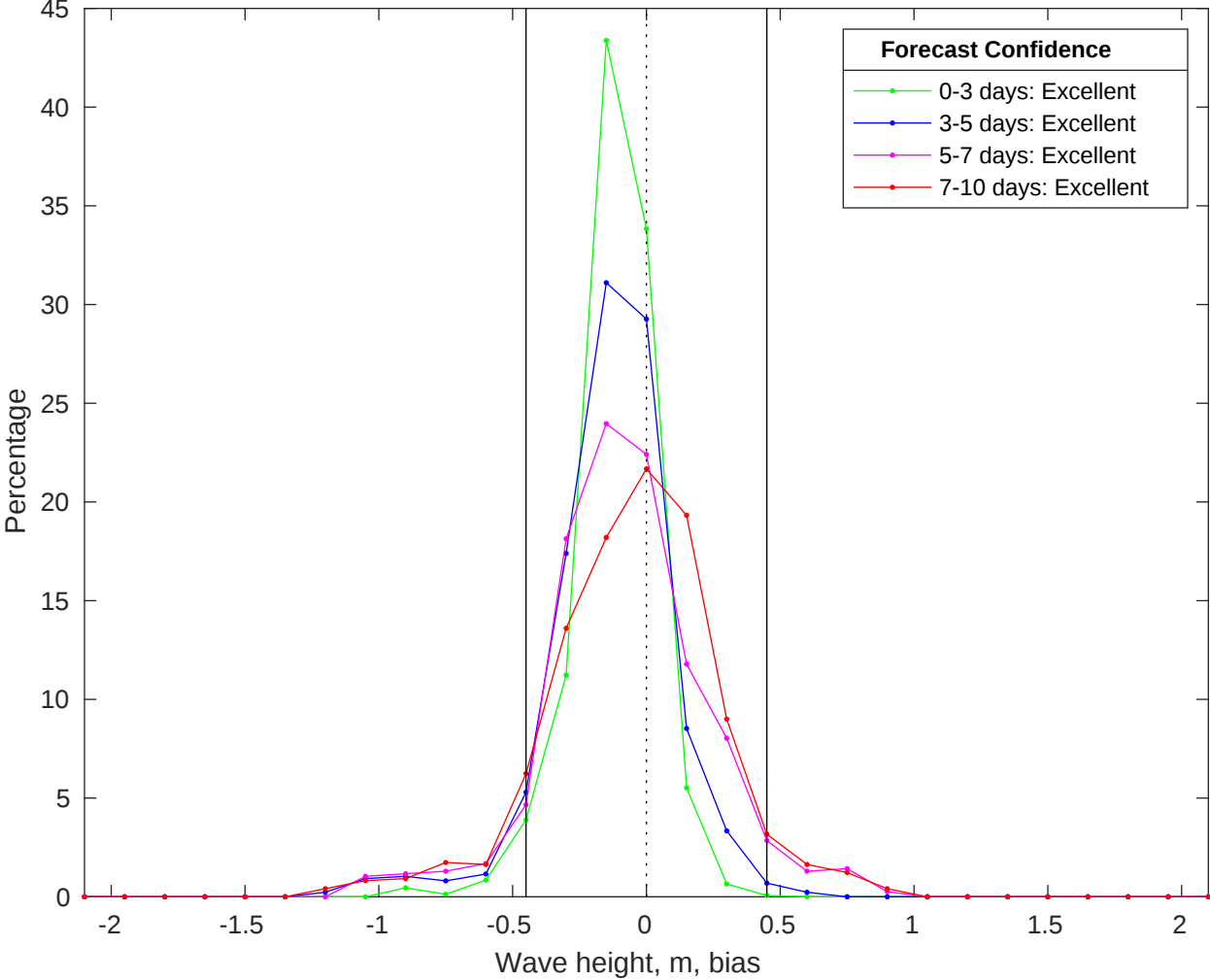
NDBC 42019 vs CMEMS Waves Bias Histogram: 20-Jun-2025
