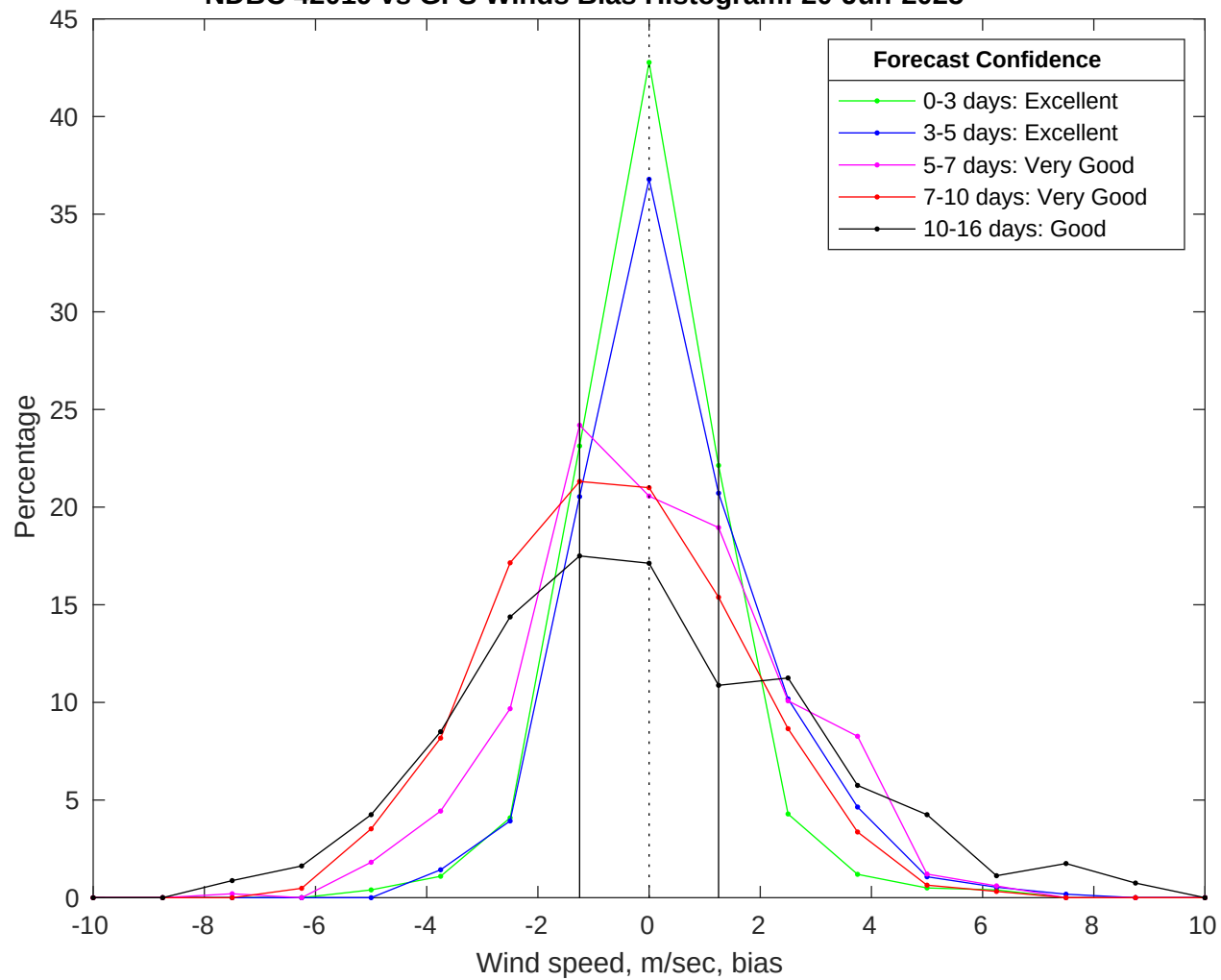
NDBC 42019 vs GFS Winds Bias Histogram: 20-Jun-2025
