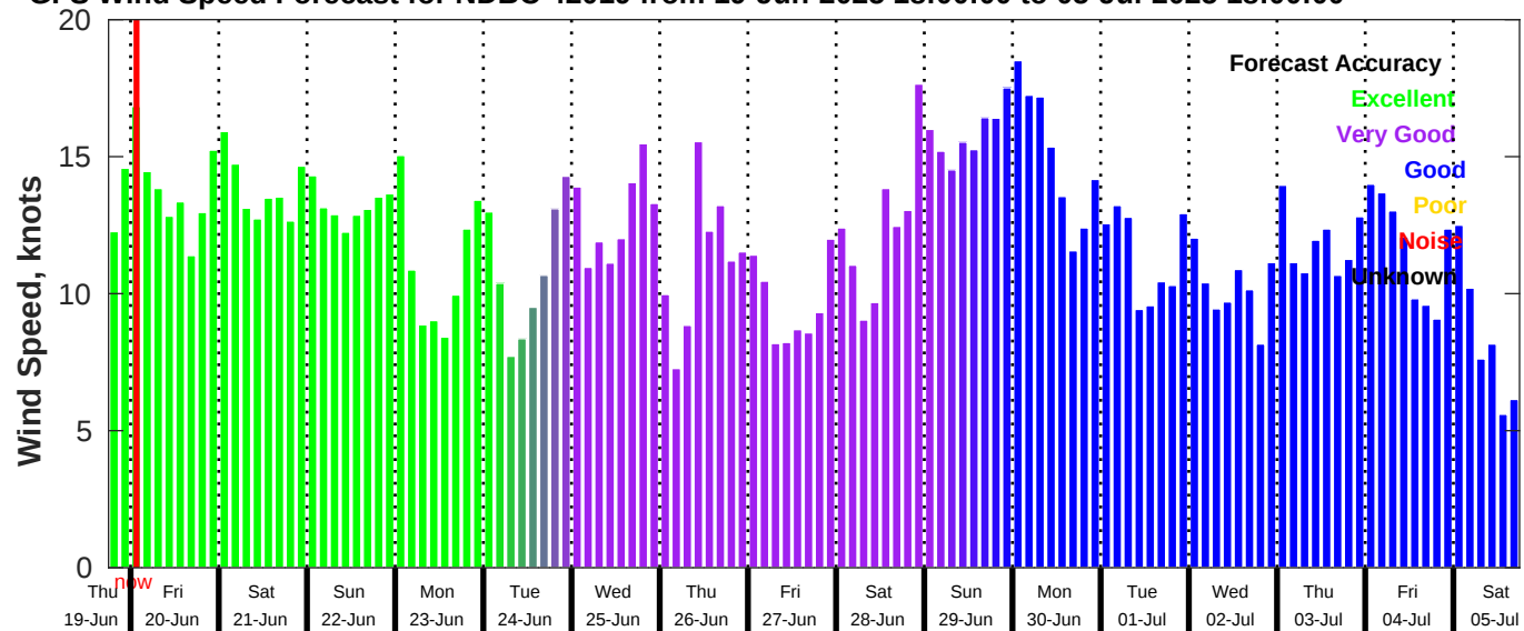
GFS Wind Speed Forecast for NDBC 42019 from 19-Jun-2025 18:00:00 to 05-Jul-2025 18:00:00
