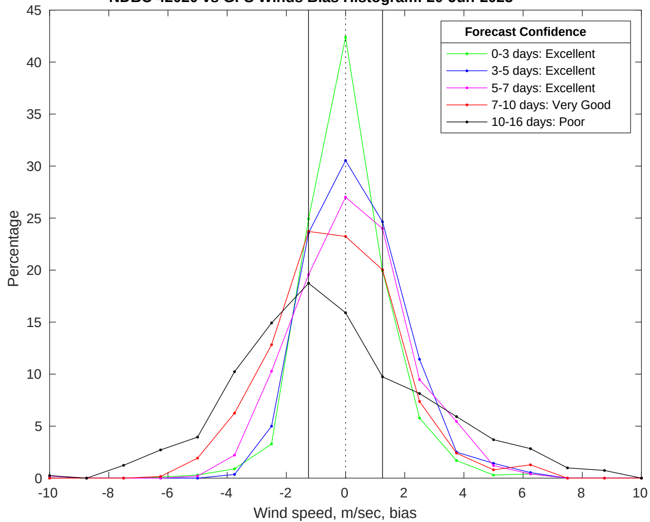
NDBC 42020 vs GFS Winds Bias Histogram: 20-Jun-2025
