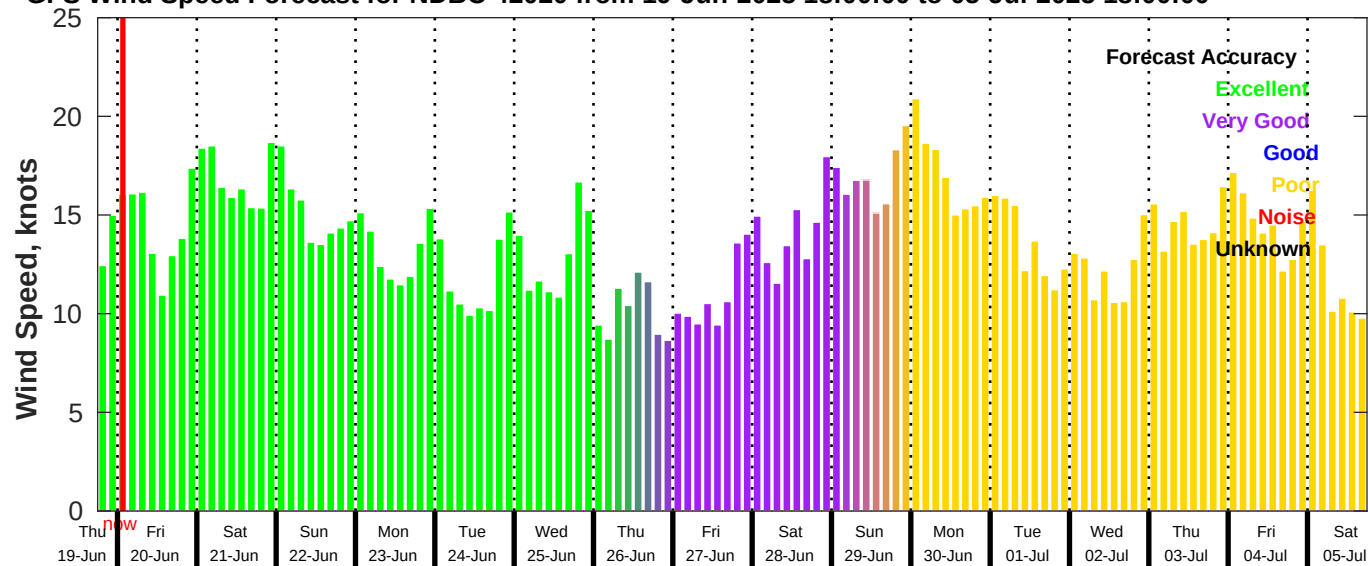
GFS Wind Speed Forecast for NDBC 42020 from 19-Jun-2025 18:00:00 to 05-Jul-2025 18:00:00
