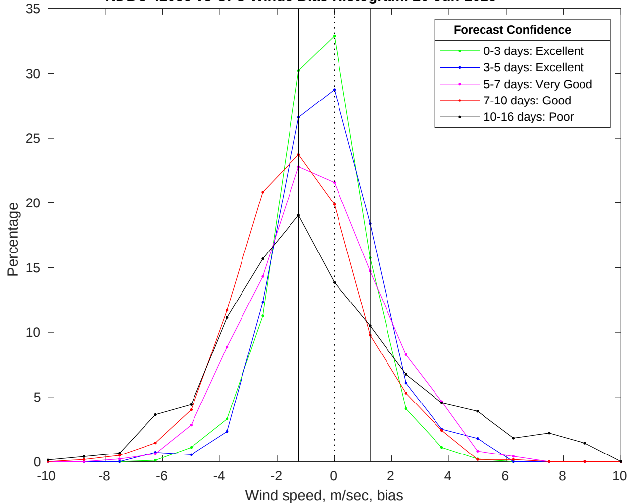
NDBC 42035 vs GFS Winds Bias Histogram: 20-Jun-2025
