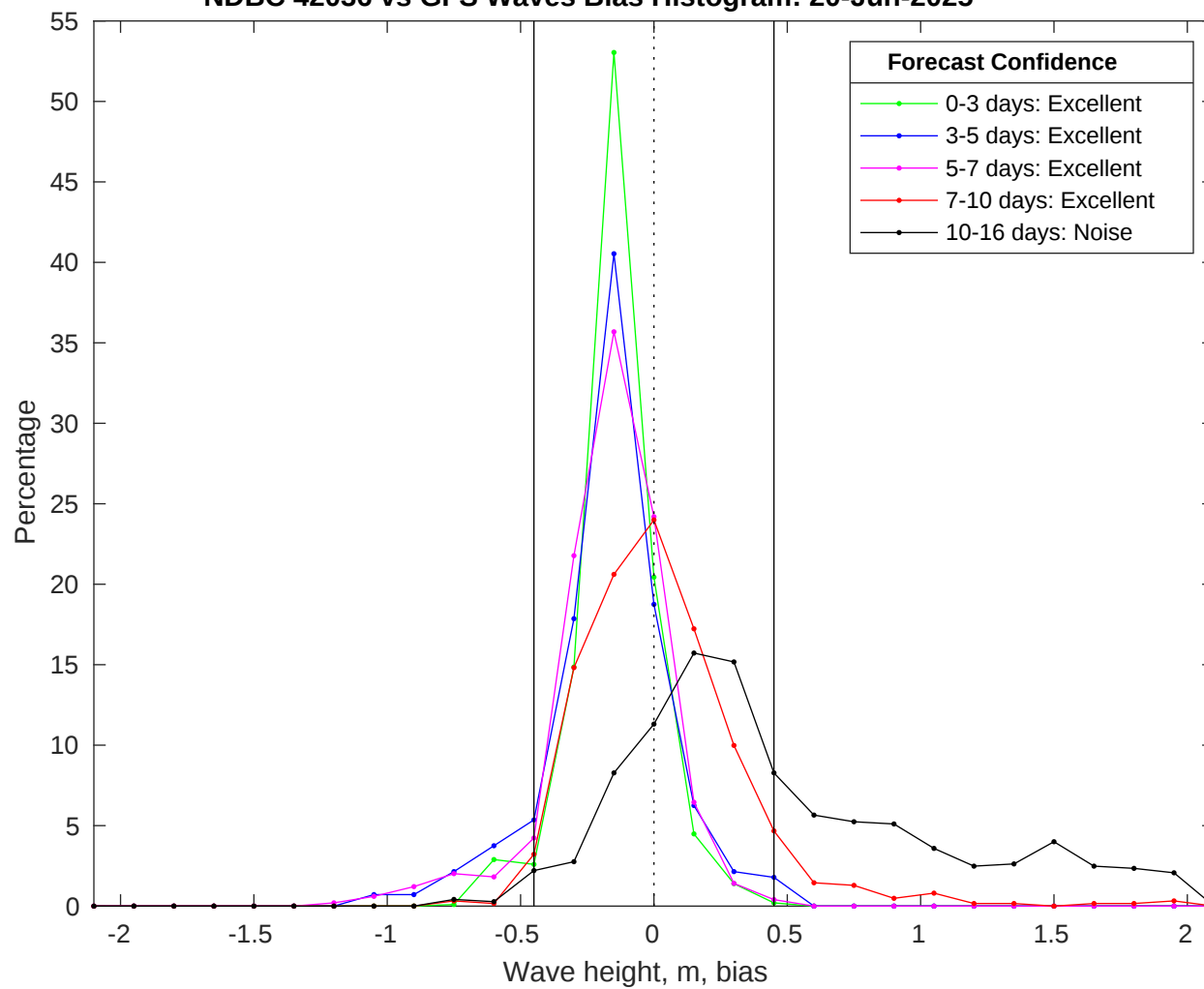
NDBC 42036 vs GFS Waves Bias Histogram: 20-Jun-2025
