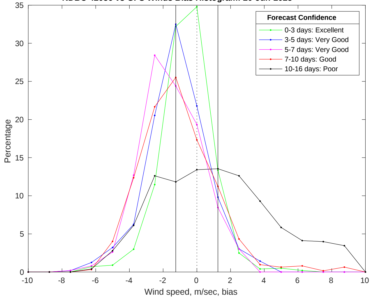
NDBC 42036 vs GFS Winds Bias Histogram: 20-Jun-2025
