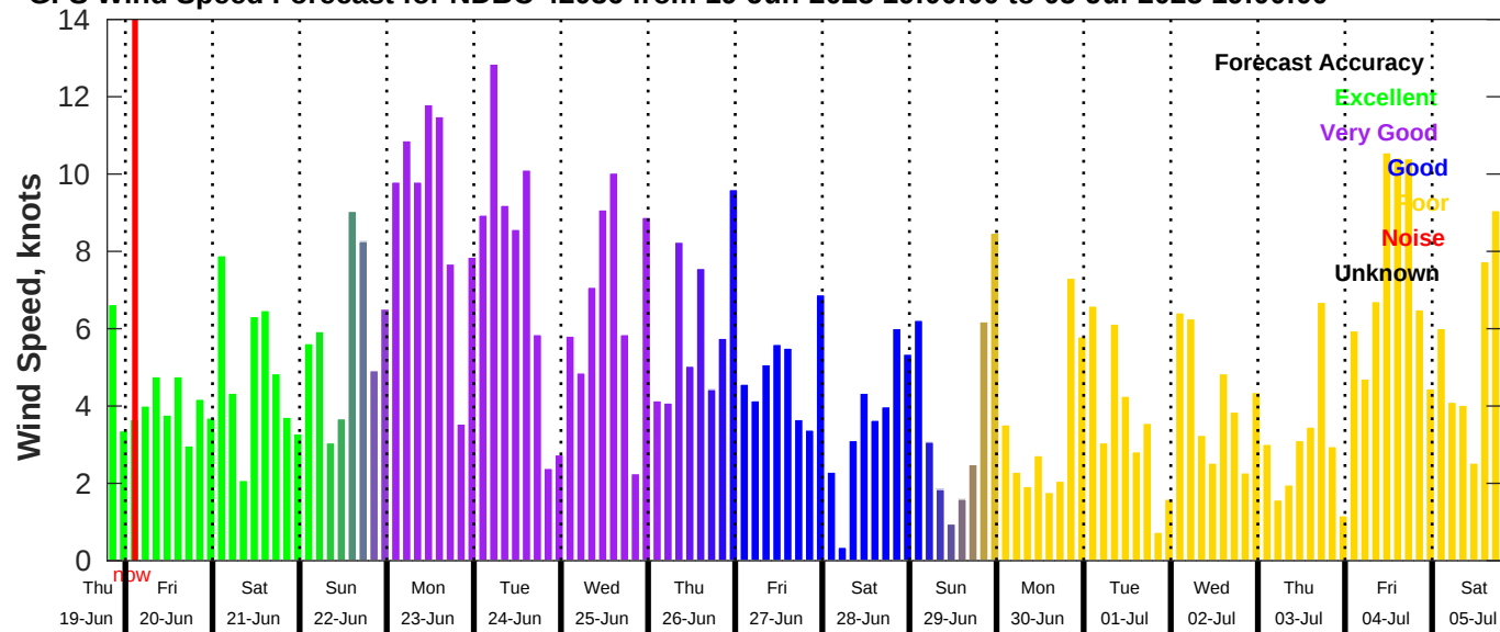
GFS Wind Speed Forecast for NDBC 42036 from 19-Jun-2025 19:00:00 to 05-Jul-2025 19:00:00
