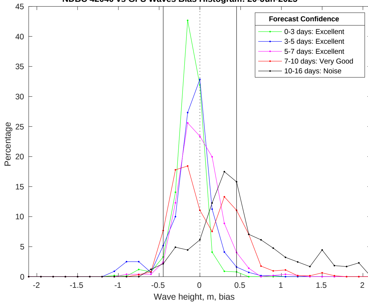
NDBC 42040 vs GFS Waves Bias Histogram: 20-Jun-2025
