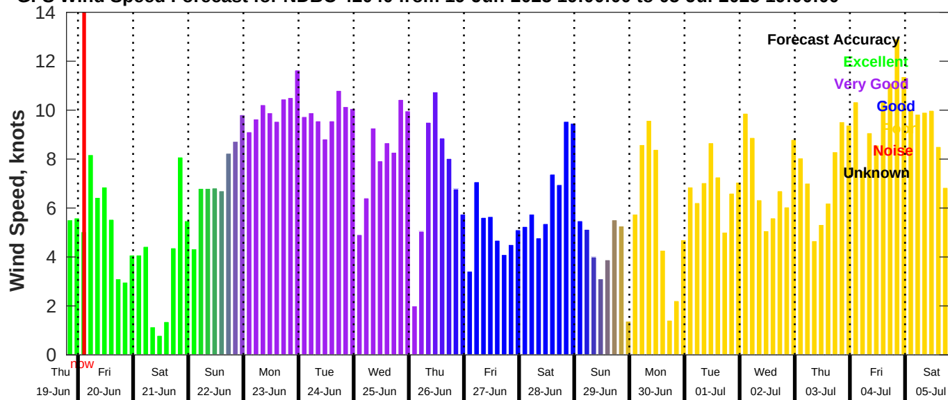
GFS Wind Speed Forecast for NDBC 42040 from 19-Jun-2025 19:00:00 to 05-Jul-2025 19:00:00
