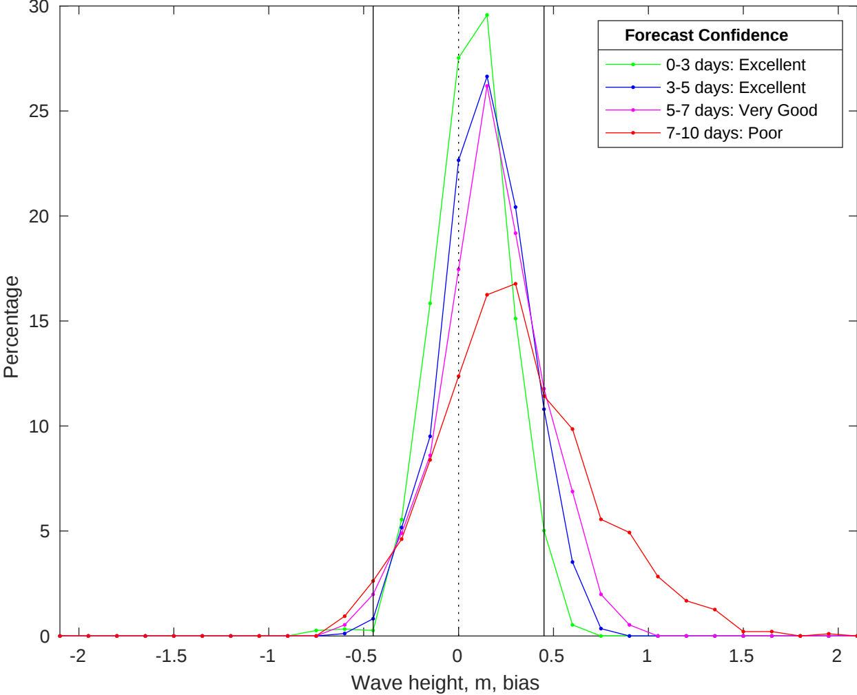
NDBC 46011 vs CMEMS Waves Bias Histogram: 20-Jun-2025
