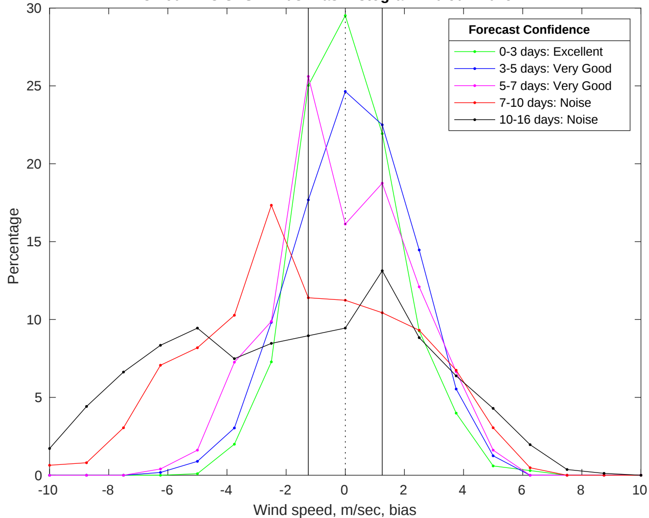
NDBC 46011 vs GFS Winds Bias Histogram: 20-Jun-2025
