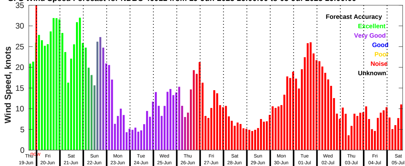
GFS Wind Speed Forecast for NDBC 46011 from 19-Jun-2025 16:00:00 to 05-Jul-2025 16:00:00
