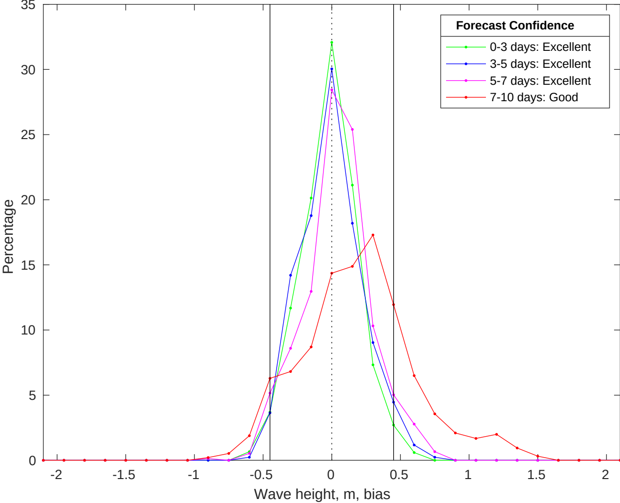
NDBC 46028 vs CMEMS Waves Bias Histogram: 20-Jun-2025
